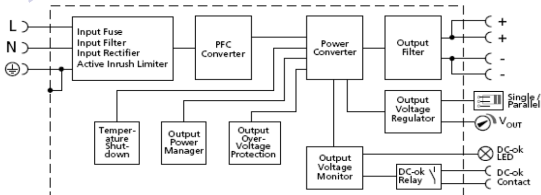
Functional diagram
