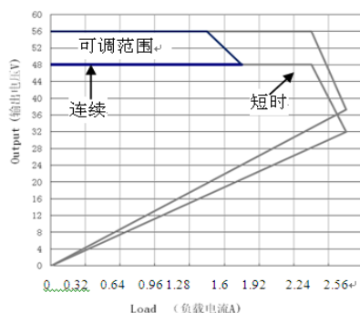
图 3-1-2 Output V-I curve (输出负载特性曲线)
