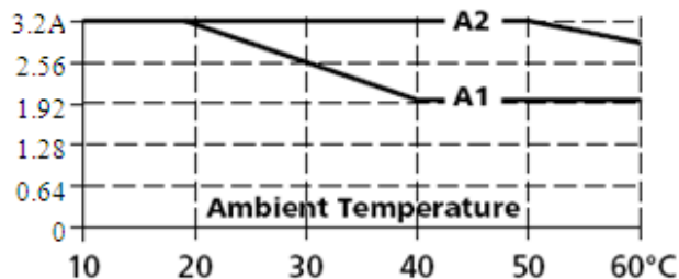
Output Current
