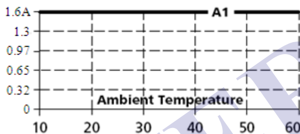
Output Current
